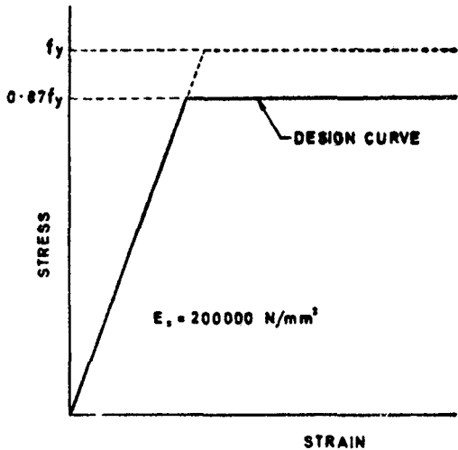
FIG. 2 STRESS-STRAIN CURVE FOR MILD STEEL
